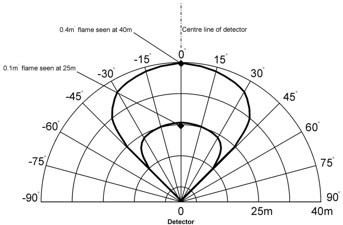
Fig 3 Detector Field of View Plot
